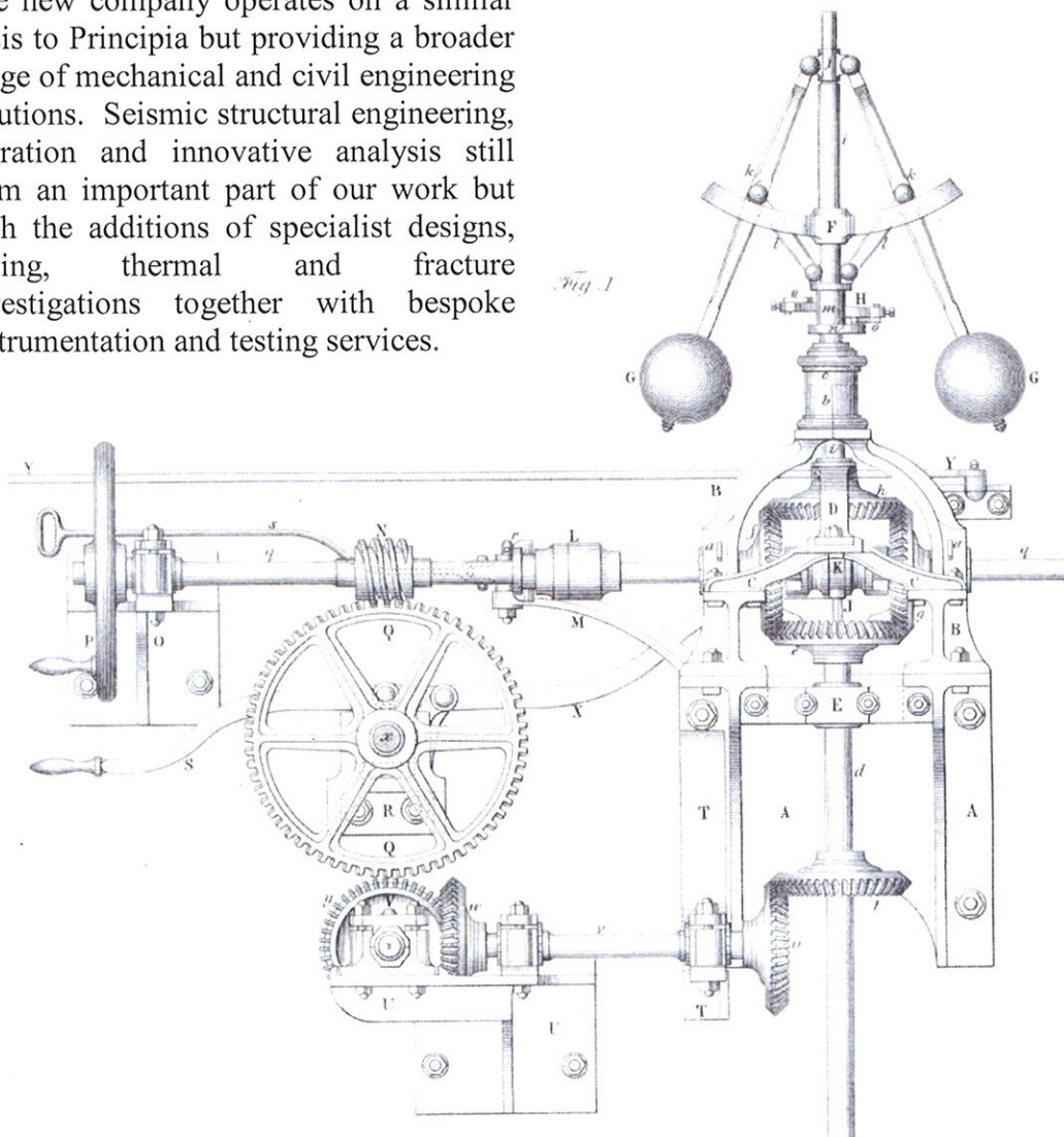
The governor for the Greenock Waterwheel, 1843.
